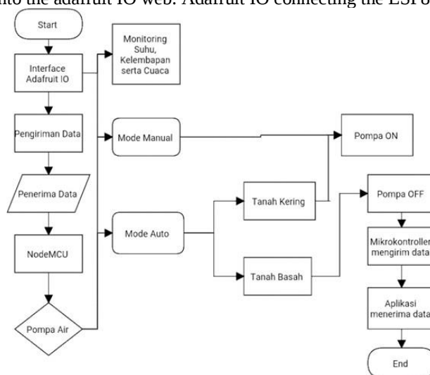
Figure 4 Software Flowchart
